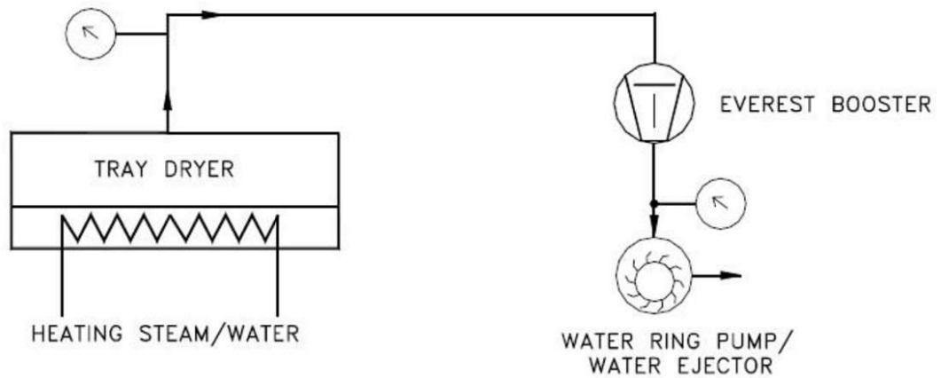
Fig: Vacuum Tray Dryer installation for Low residual moisture requirement – Ideally used in Pharmaceutical, Food & Chemical Drying.
