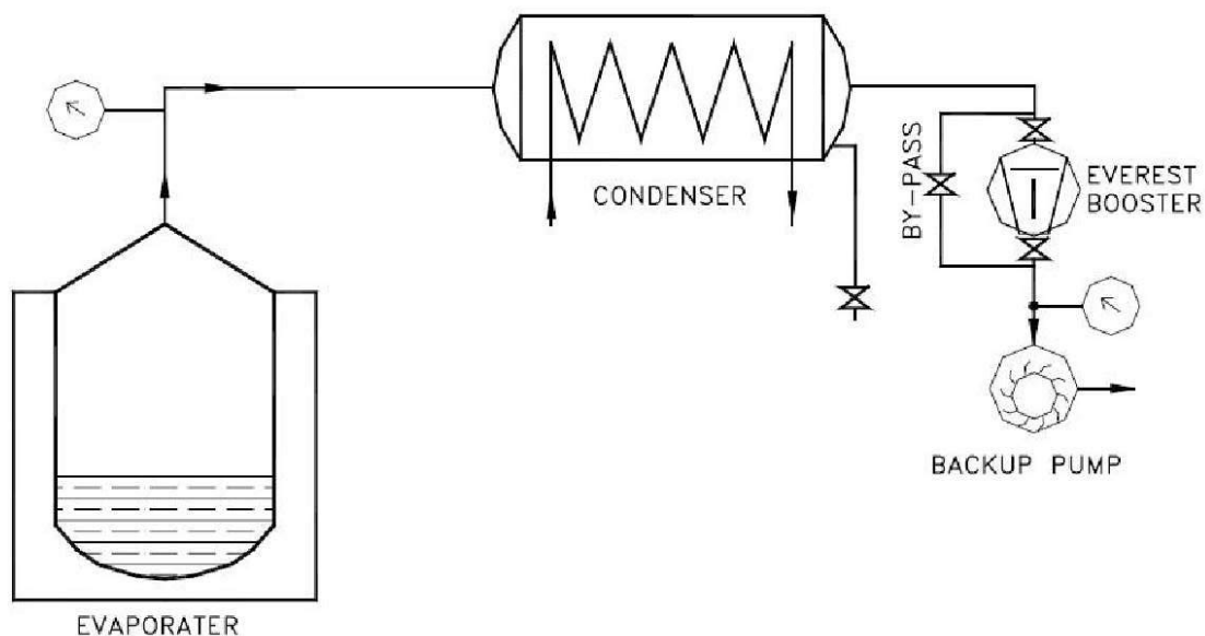
Fig: Booster arrangement with External Bypass for Solvent Recovery Application requiring high vacuum at final stages.
