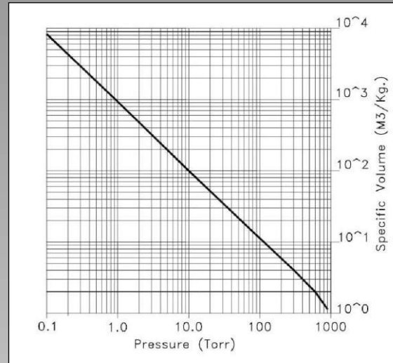
Graph: Specific volume of water vapour at various pressure
