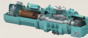
CANNED MOTOR MECHANICAL VACUUM BOOSTERS
